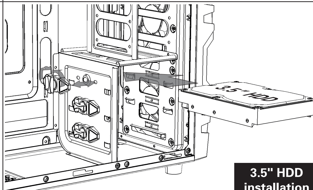
3.5" device installation
